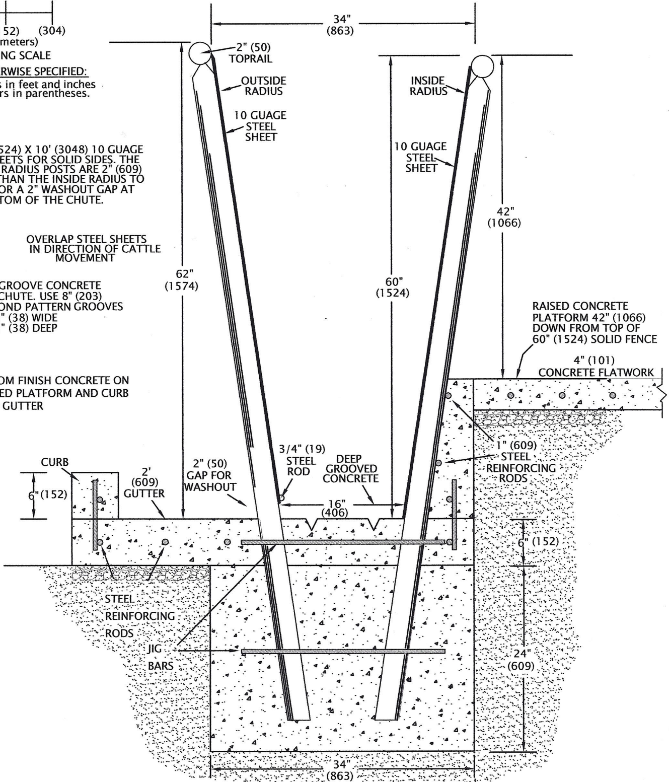
V-SHAPED SINGLE FILE CHUTE WITH RAISED CONCRETE PLATFORM, WASHOUT GUTTER AND CURB
